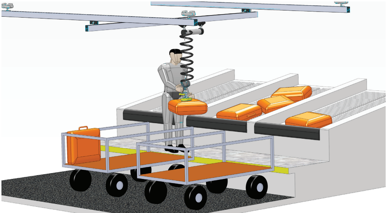
Loading baggage from chutes to carts.
